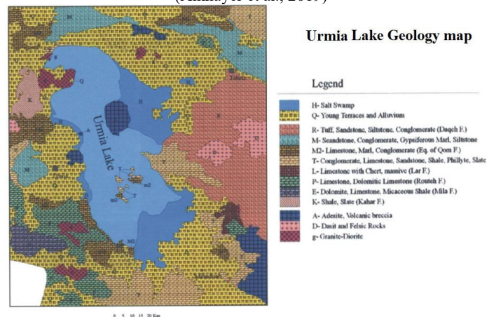
Fig. 4 Geological Map of Urmia Lake region (Azarafza & Mokhtari, 2013)
