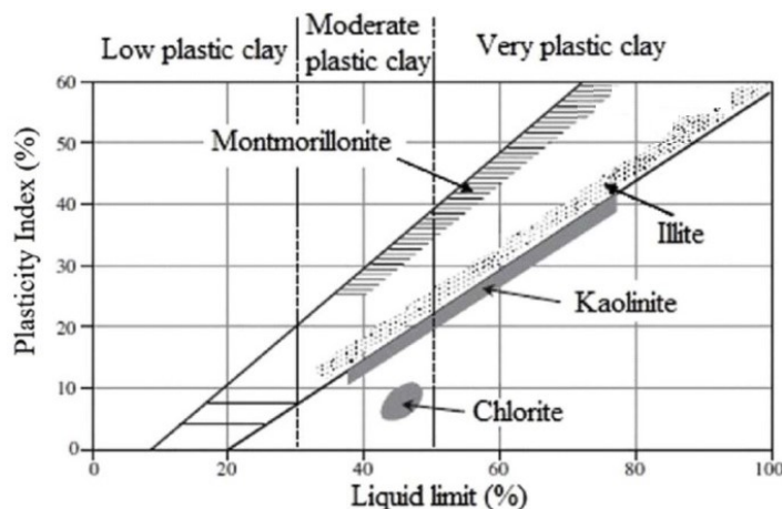
Fig. 2 Clay minerals position on the Holtz & Kovacs (1981) diagram
